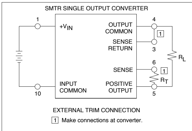
FIGURE 1: TRIM CONNECTION 1, 2, 3
