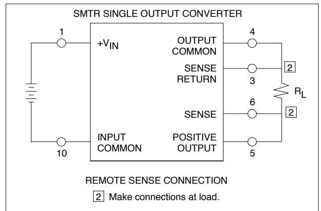
FIGURE 2: REMOTE SENSE 2, 3
