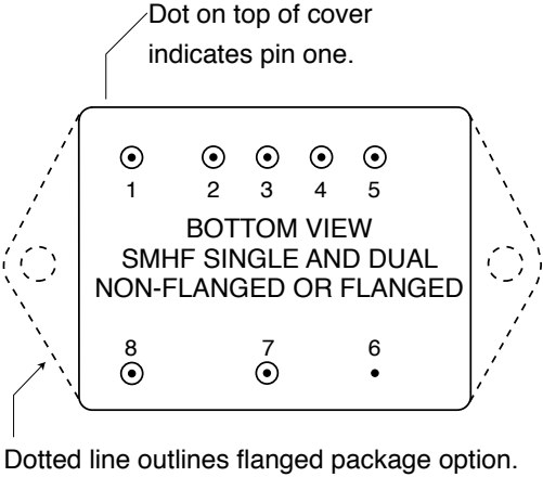
FIGURE 3: PIN OUT
