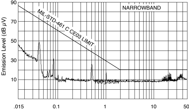
Frequency (MHz), 28 V IN SMHF2805S with Interpoint SFMC28-461 EMI Filter, Representative of the SMHF Series of DC-DC Converters FIGURE 6
