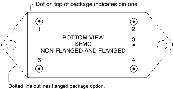
FIGURE 2: PIN OUT
