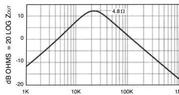
Typical Output Impedance (Z) With Input Shorted FIGURE 5
