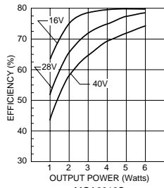
Typical Performance Curves: 25°C Tc, 28 VDC Vin, 100% load, unless otherwise specified.
